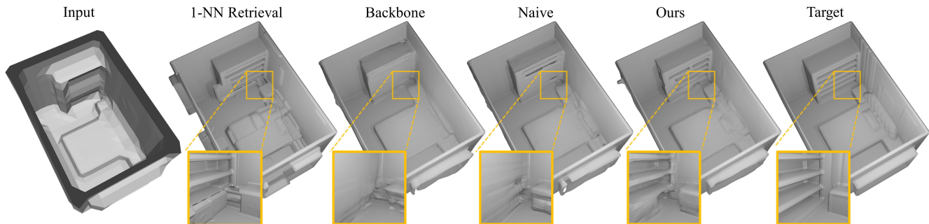
Figure 7: Qualitative evaluation of our method ( Ours ) in comparison to 1 st nearest neighbor retrieval ( 1-NN Retrieval ), our refinement network without retrievals ( Backbone ) and naive fusion of retrieved approximations during refinement ( Naive ).
