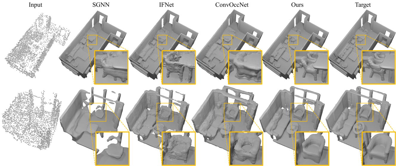
Figure 6: Point cloud to surface reconstruction on 3DFront (top) and Matterport3D (bottom) datasets. Our approach captures more coherent structures and object details.
